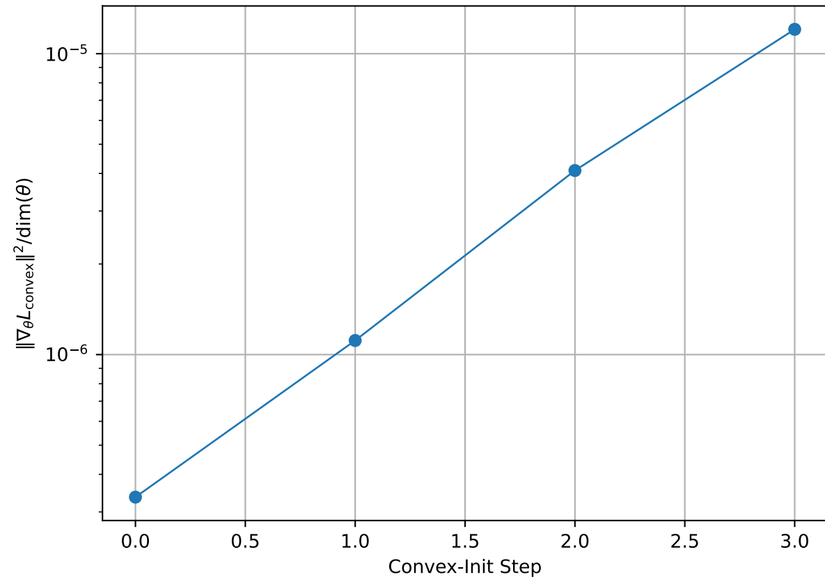
Barren Plateau Diagnostic: Gradient Norm (Convex Init)
